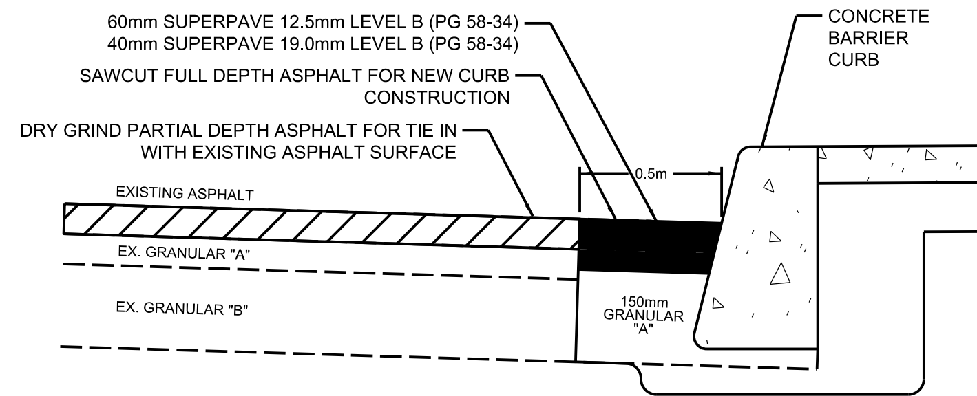
DETAIL 1: ROAD REINSTATEMENT
